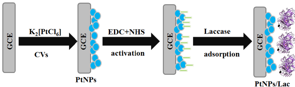
Scheme 1. Construction of the PtNPs/laccase modified electrodes.
