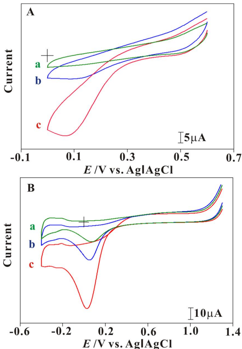
Figure 2. (A) CVs recorded at a laccase modified electrode in 0.1M PBS (pH 7.0 containing 1 mM ABTS ) saturated with nitrogen (curve a), ambient air (curve b) and oxygen (curve c). Scan rate 100 \text{ mVs}^{-1} in the potential range of 0.6 to 0 V. (B) CVs recorded at a PtNPs modified electrode in 0.1M PBS (pH 7.0 containing 1 mM ABTS ) saturated with nitrogen (curve a), ambient air (curve b) and oxygen (curve c). Scan rate 100 \text{ mVs}^{-1} in the potential range of 1.3 to -0.4 V.
