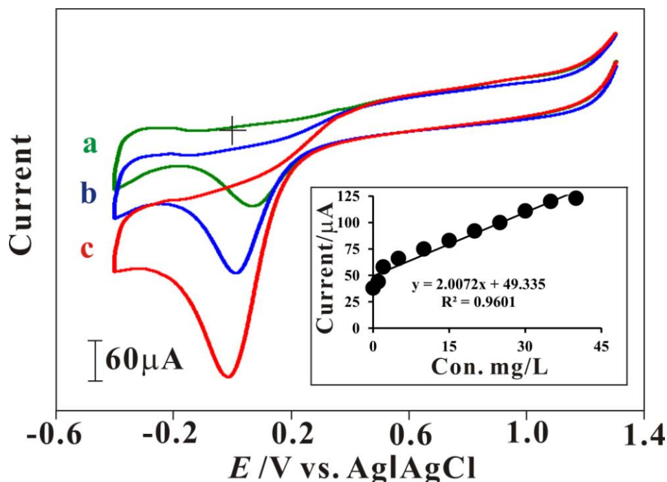
Figure 3. CVs recorded at a PtNPs/laccase modified electrode in 0.1M PBS (pH 7.0 containing 1 mM ABTS ) saturated with nitrogen (curve a), ambient air (curve b) and oxygen (curve c). Scan rate 100 \text{ mVs}^{-1} in the potential range of 1.3 to -0.4 V. Inset shows a current vs. concentration plot of oxygen at PtNPs/laccase electrode.
