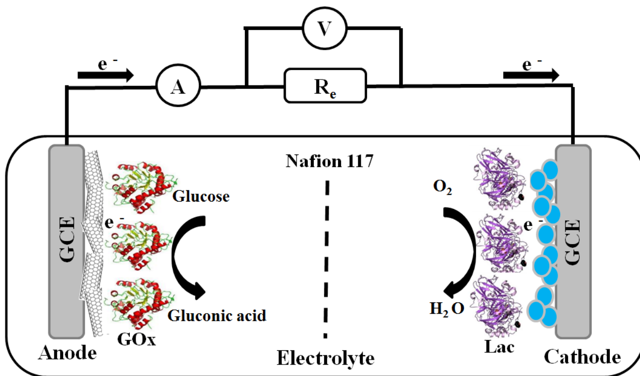
Scheme 2. The configuration biofuel cell with bioanode and biocathode.
