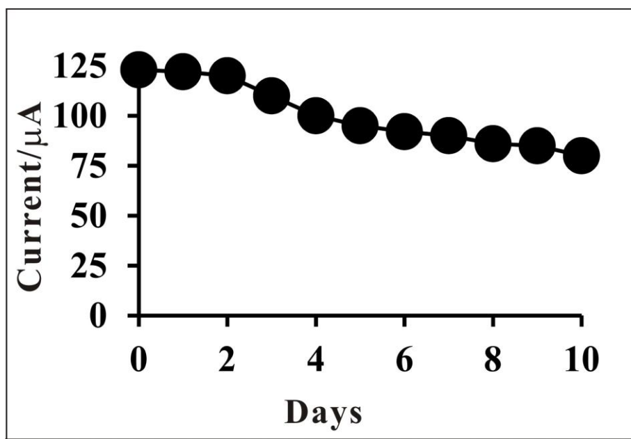
Figure 4. Reduction oxygen peak current of PtNPs/laccase modified electrodes stored in pH 7.0 PBS at 4 °C for 10 consecutive days.
