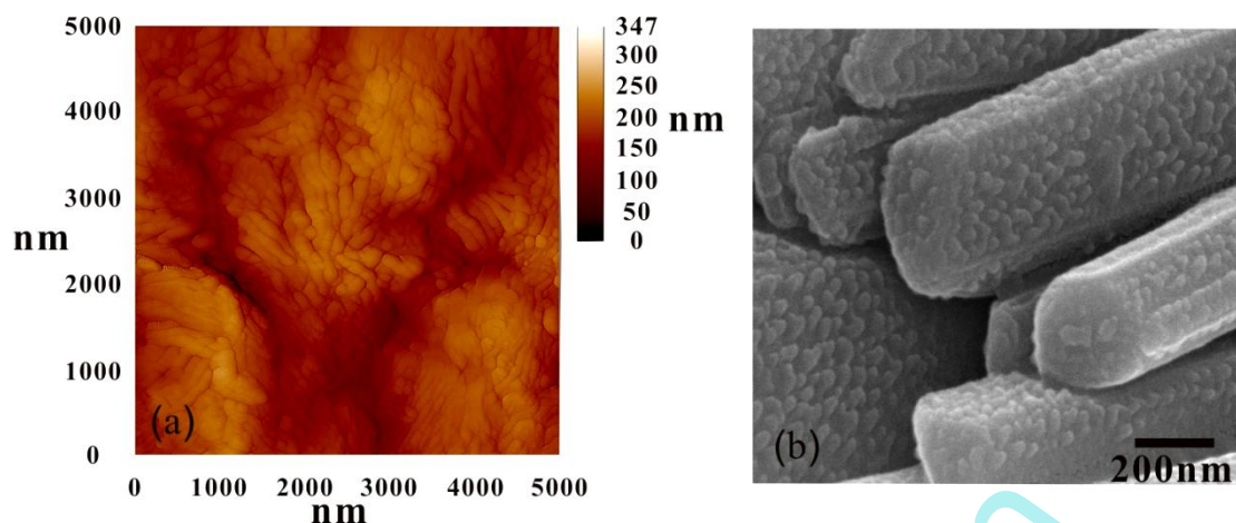
Figure 3. a) AFM image of Nafion/Pd-GOx and b) FE-SEM image of Nafion/Pd-GOx.
