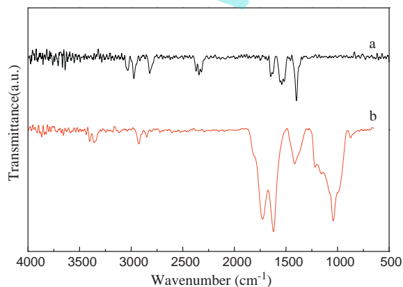
Fig. 1. FTIR spectra of MWCNT and GO.
